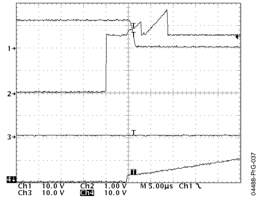
Figure 38. Timing Waveforms Associated with an Overvoltage Fault (Ch1 = GATE; Ch2 = OV; Ch3 = PWRGD; Ch 4 = SPLYGD)
